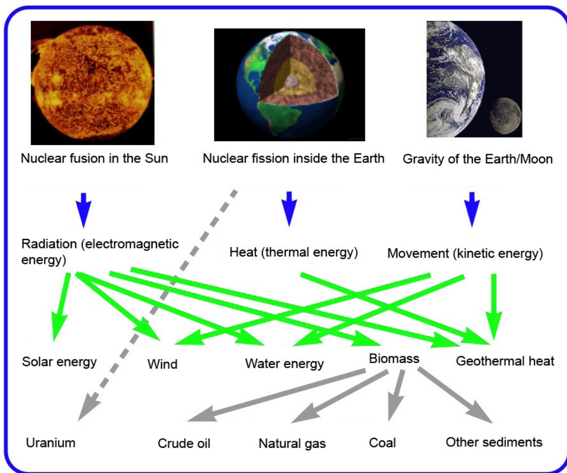
Pic. 1.2: Usable energy spectrum
